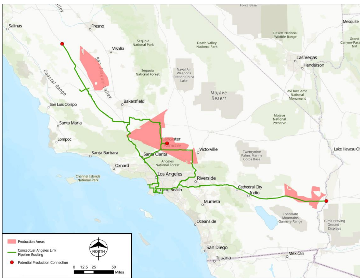
Figure 12. Conceptual Production Areas and Pipeline Routing
