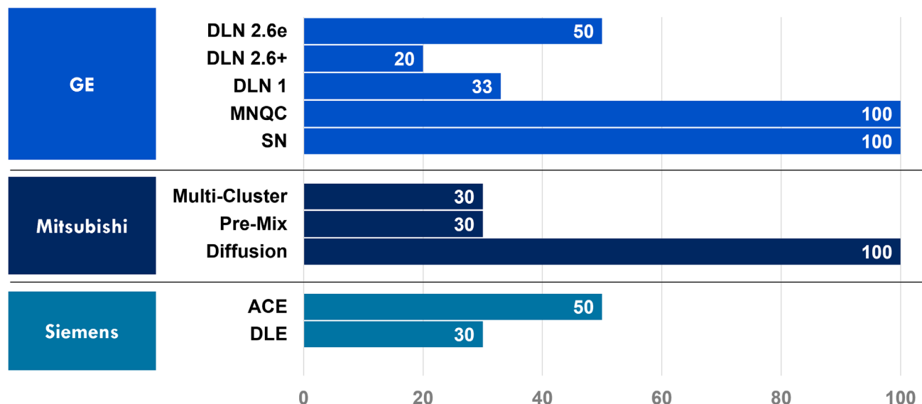
Figure 15: Current H2 Capability across Major Power Manufacturer Models (% by Volume)
